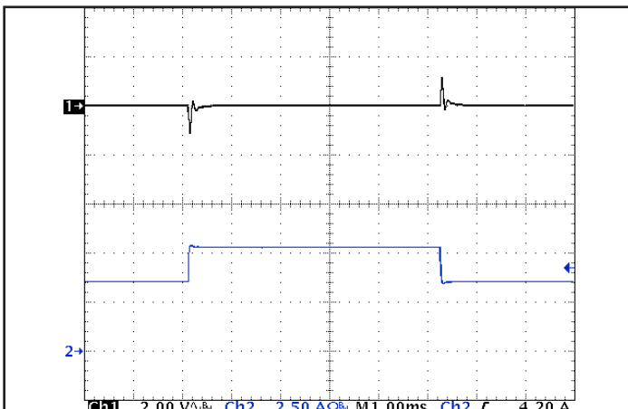
Figure 5: Output voltage response to step-change in load current (50 %-75 %-50 % of I_{out(max)} ; dI/dt = 0.1 A/\mu s ). Load cap: 1 uF ceramic capacitor. Ch 1: V_{out} , Ch 2: I_{out} .
