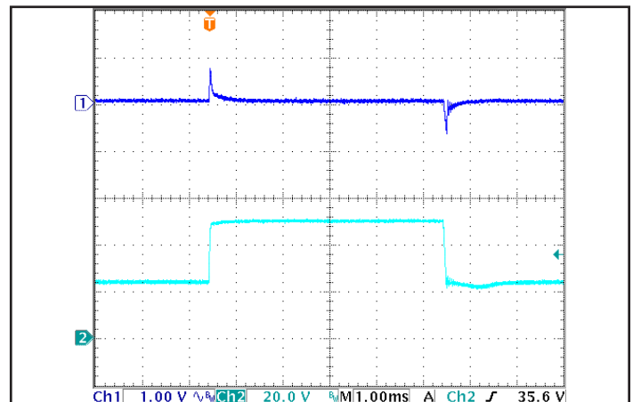
Figure 6: Output voltage response to step-change in input voltage (nominal to maximum, 250 V/ms). Load cap: 15 \mu F tantalum and 1 \mu F ceramic capacitors. Ch 1: V_{out} , Ch 2: V_{in} .
