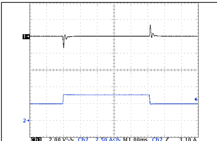
Figure 5: Output voltage response to step-change in load current (50 %-75 %-50 % of I out (max); dI/dt = 0.2 A/μs). Load cap: 1 uF ceramic capacitor. Ch 1: V out , Ch 2: I out .
