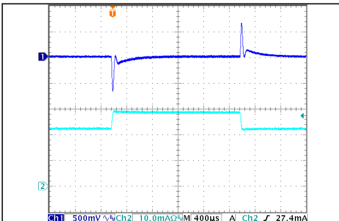
Figure 5: Output voltage response to step-change in load current (50 %-75 %-50 % of I out (max); dI/dt = 0.2 A/μs). Load cap: 1μF ceramic capacitor. Ch 1: V out , Ch 2: I out (2 A/div).
